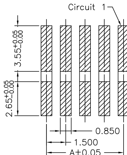
PCB LAYOUT
