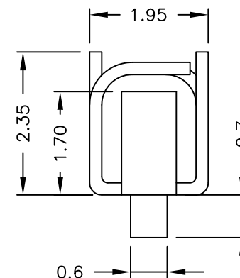
Section C-C
