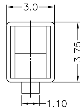
Section C-C
